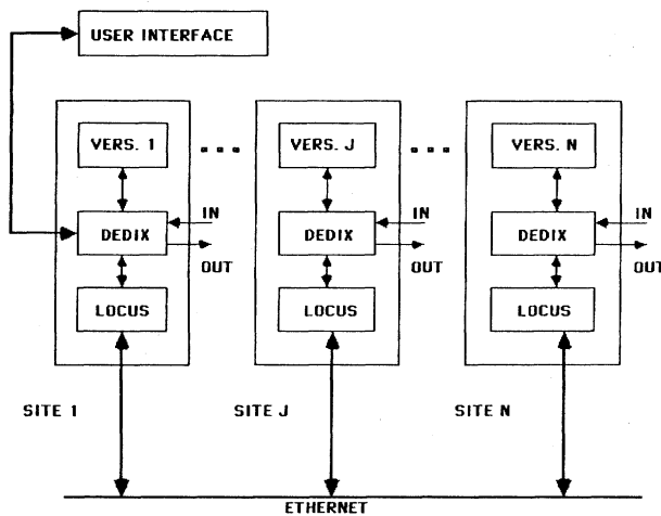
Fig. 1. DEDIX at N sites of Olympus Net.
