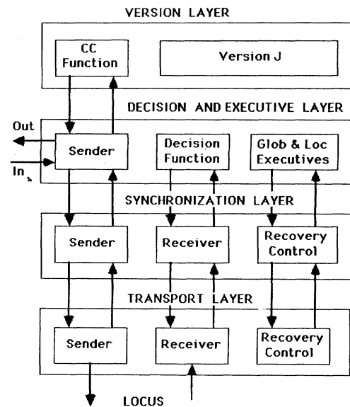
Fig. 2. Layers and entities at one site of DEDIX.
